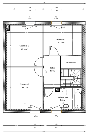
PLAN R+1
